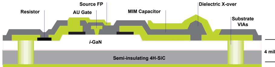
G28V3 process cross section
